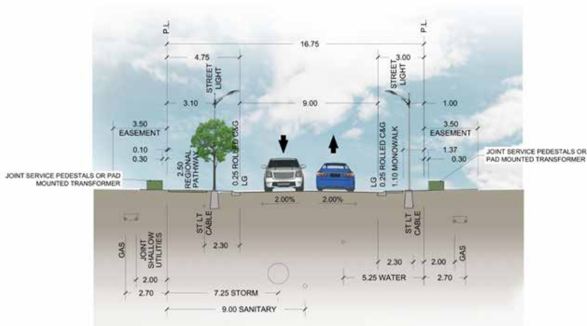
FIGURE C-5. 16.75 RESIDENTIAL
