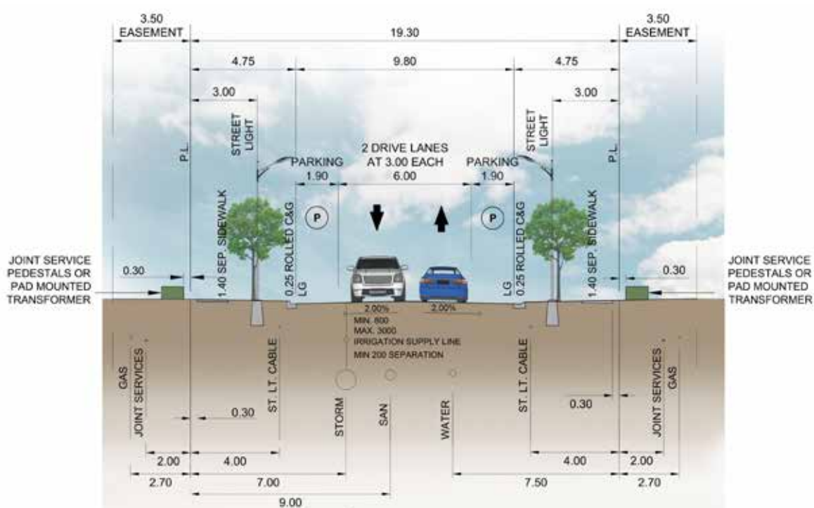
FIGURE C-4. 19.30M COLLECTOR AVENUE
