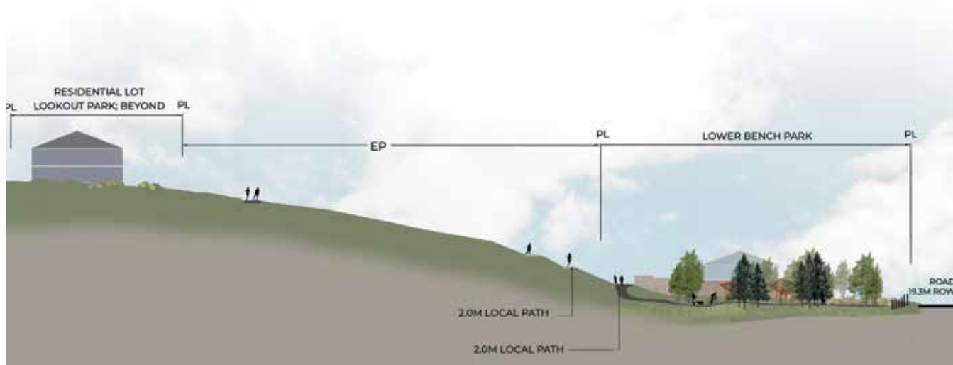
FIGURE 15. ESCARPMENT SECTION: LOWER BENCH
