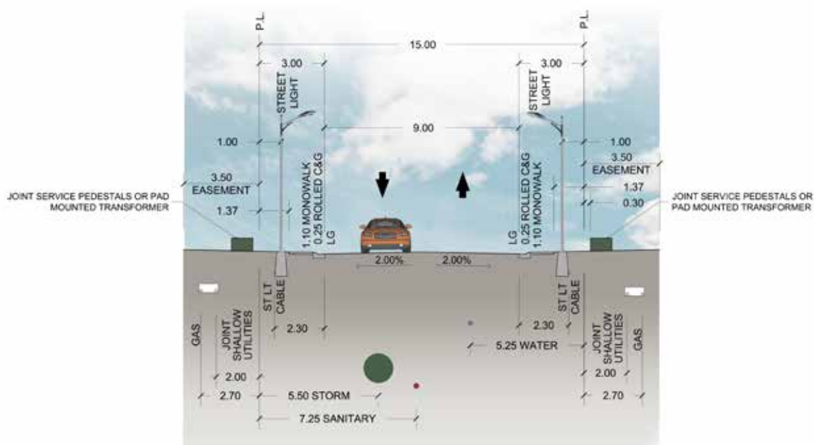
FIGURE C-6. 15.00 RESIDENTIAL
