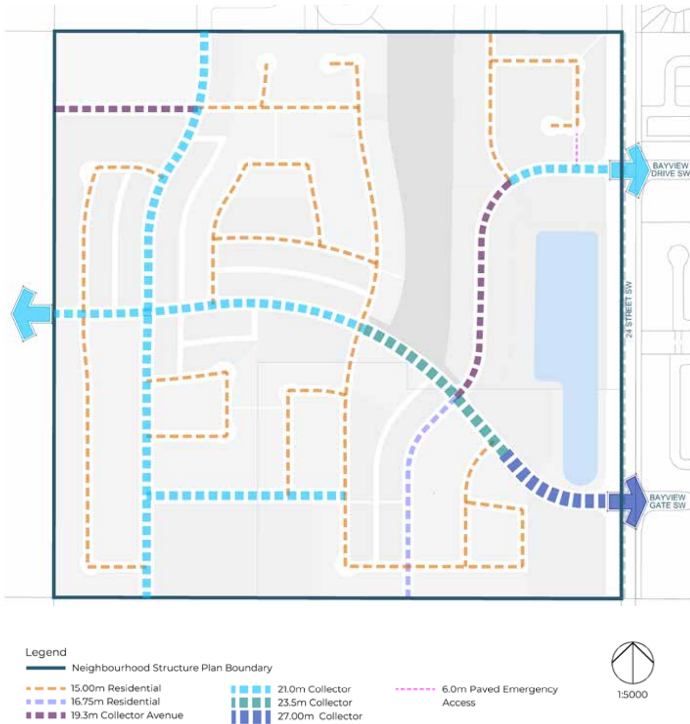
FIGURE 21. ROAD NETWORK
