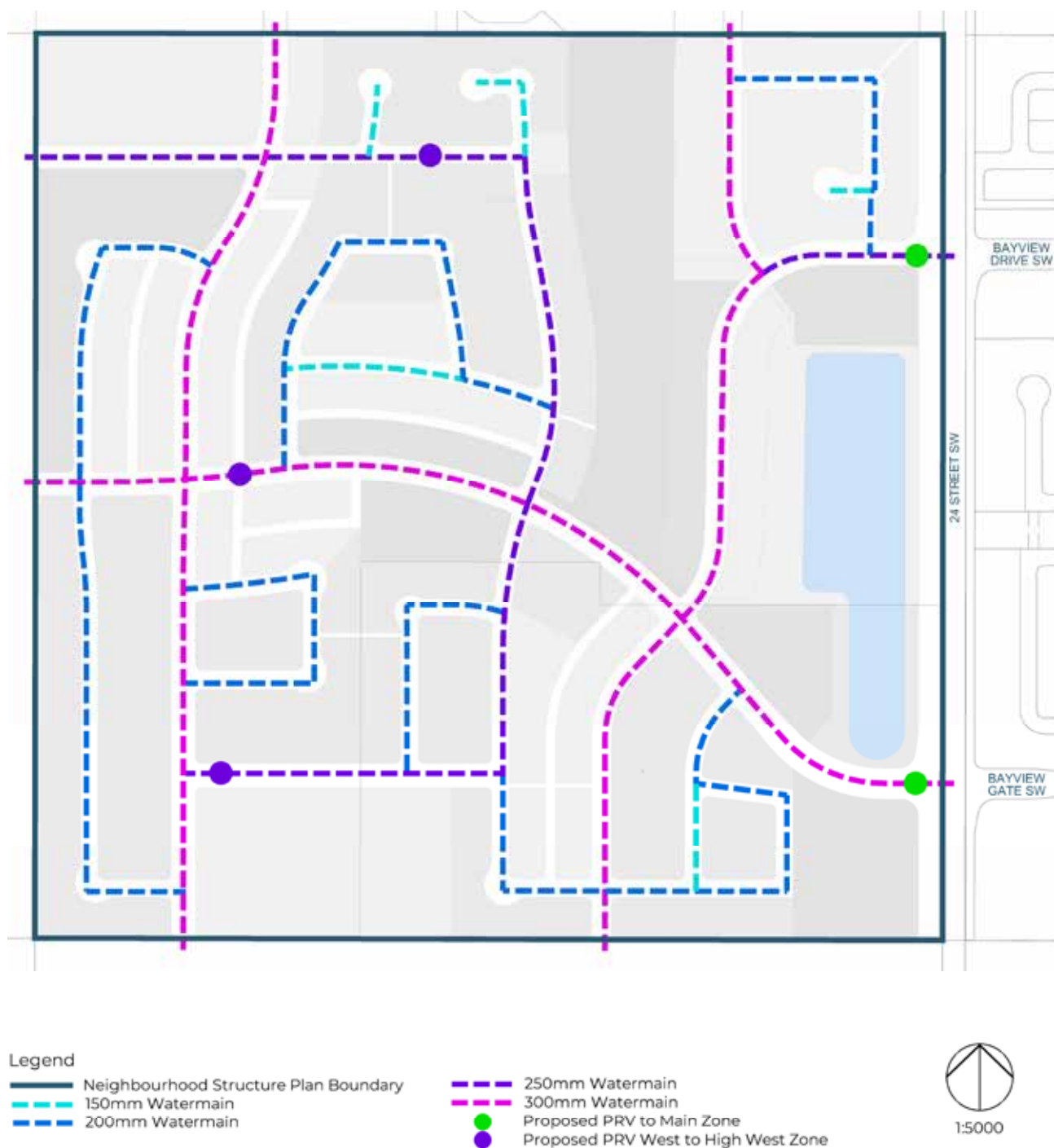
FIGURE 26. WATER SERVICING
