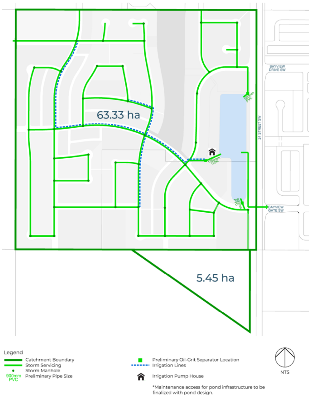
FIGURE 30. STORMWATER SERVICING
