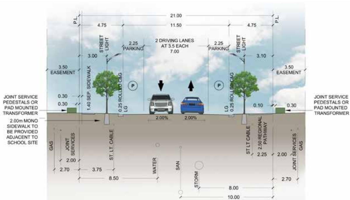
FIGURE C-3. 21.00M COLLECTOR
